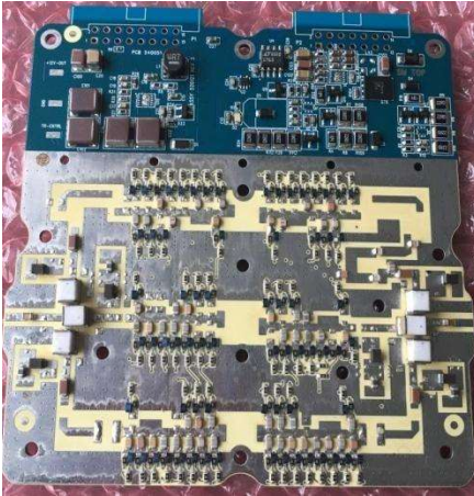
Control Board
